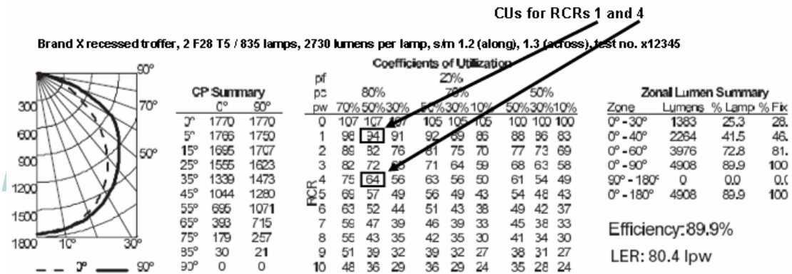
Figure 4-1 Interior Luminaire TER Calculation, CU Determination
