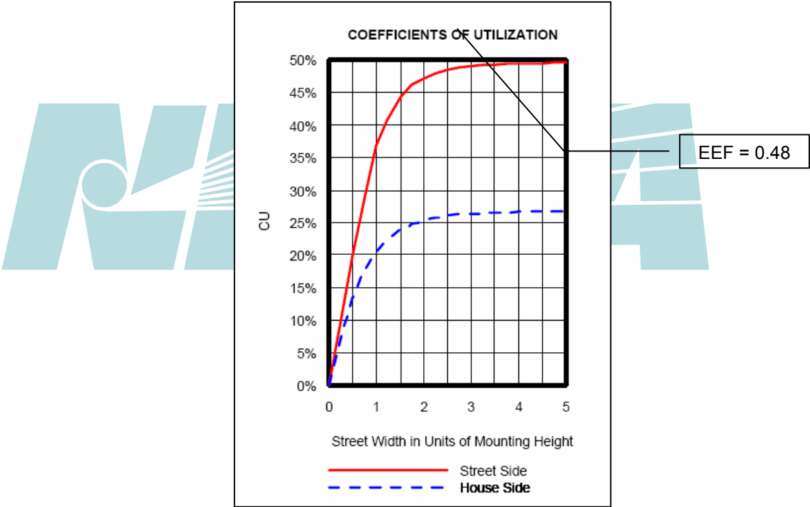
Figure 4-2 Exterior Luminaire TER Calculation, CU Determination
